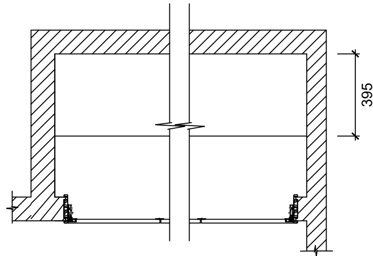
OPK Bi-fold Door Rebated Door Jamb Top View
