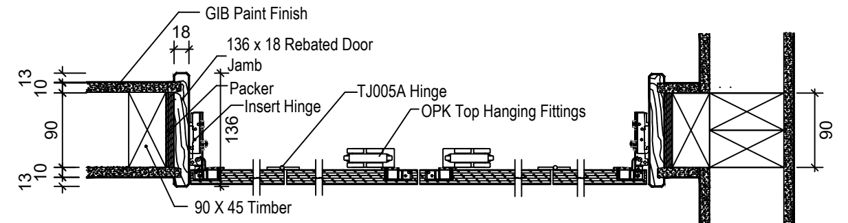
Bi-fold Door Rebated Door Jamb Top View Details Drawing
